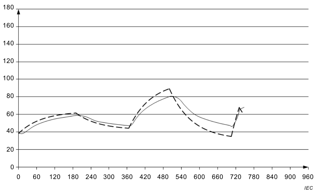
Figure H.1 – Hot-spot temperature response to step changes in the load current
