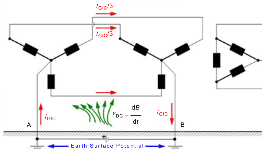
Figure L.1 – GIC flow into a power transformer
